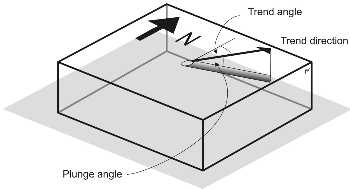
Figure 3: Trend and plunge of a linear geological feature.
