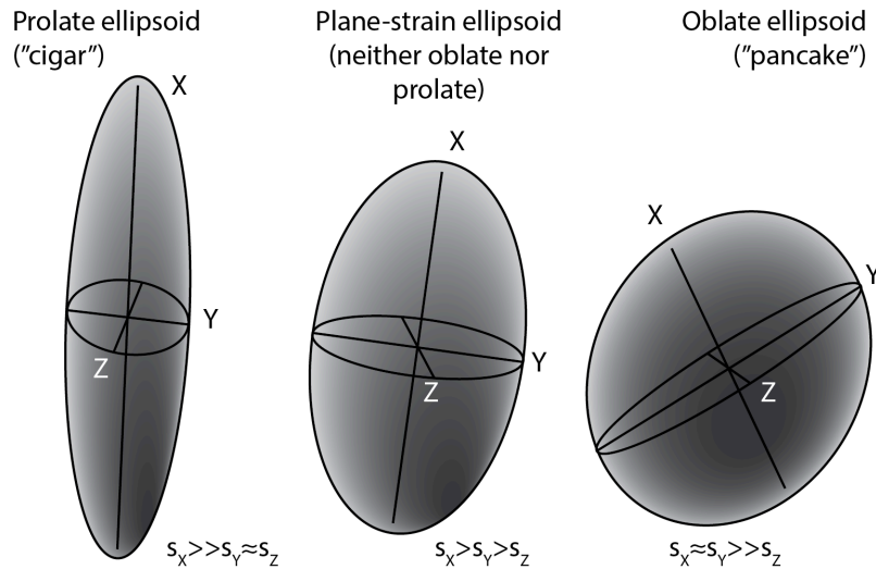
Figure 7: A range of strain ellipsoid shapes at constant volume.
