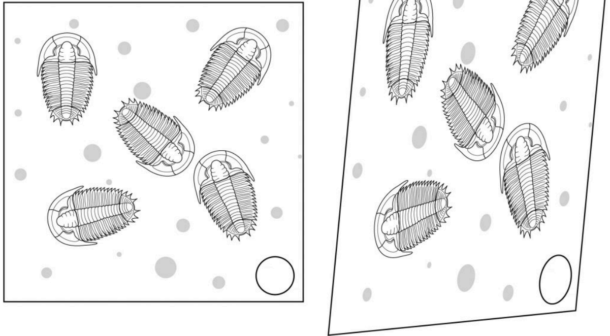
Figure 3. Strain affecting variably oriented trilobites. Note that each fossil is affected differently, depending on its initial orientation, but the strain is nonetheless homogeneous, as shown by the ellipses. Trilobite image after Gon, S.; www.trilobites.info ; Downloaded 2012 Dec 17.
