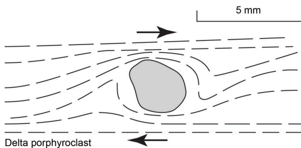
Figure 9. Sigma and delta structures.
