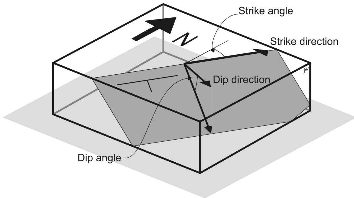
Figure 4. Strike, dip, and dip-direction of a plane.
