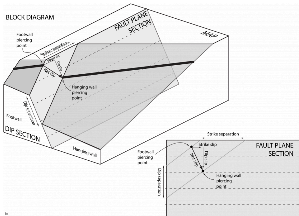
Figure 5. Piercing points on a linear feature uniquely define slip.
