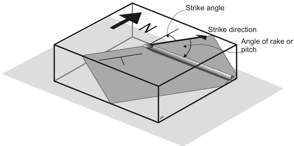
Figure 6: Rake of a linear feature in a planar feature.
