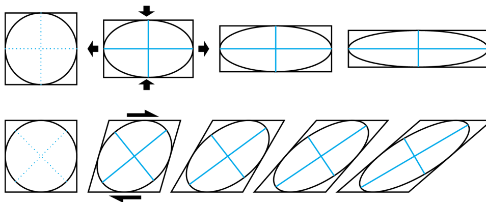
Figure 9. Top: Coaxial or pure strain. Note that the strain axes keep their directions constant relative to the material being deformed. Bottom: Simple shear, one type of noncoaxial strain history. Note that the strain axes rotate over time relative to the material being deformed.
