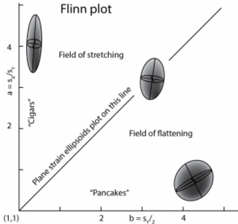
Figure 8: Flinn plot for constant-volume strain ellipsoids
