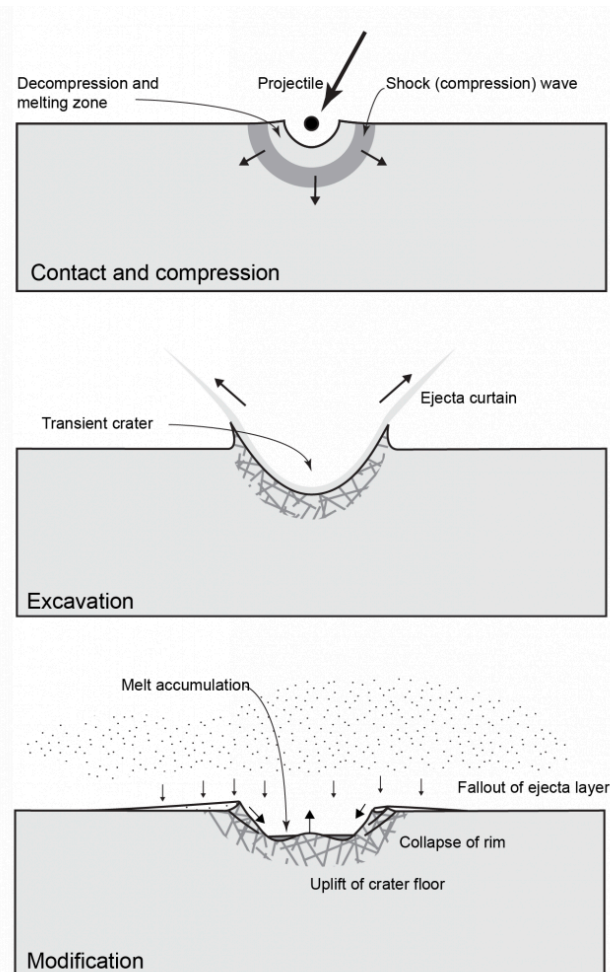
Figure 2. Three stages of crater development.
